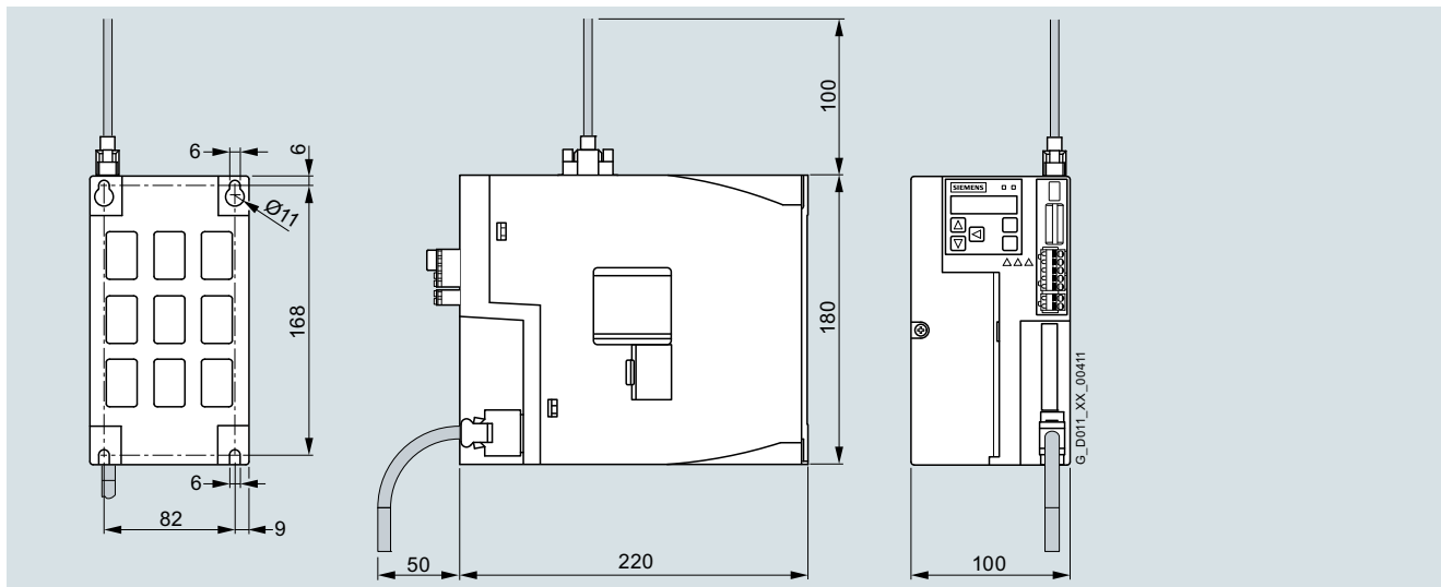
SINAMICS V90, 380 ... 480 V 3 AC, frame size FSB
