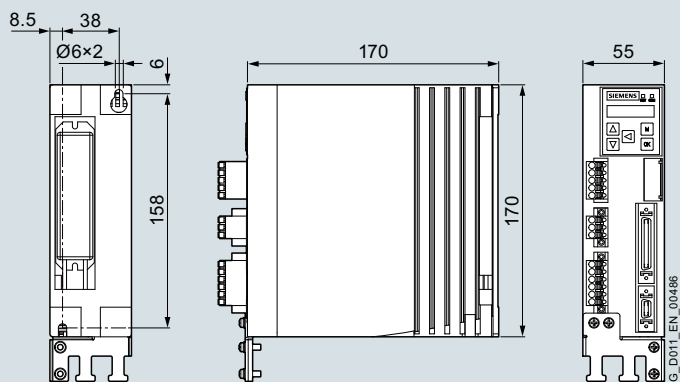
SINAMICS V90, 200 ... 240 V 1 AC/3 AC, frame size FSB
