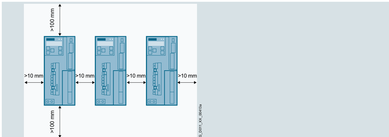
Mounting clearances
