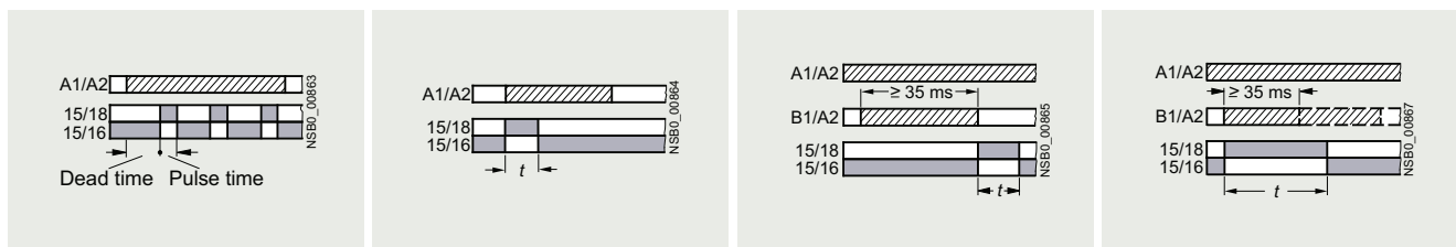
-- 7PV1558 Clock-pulse, starting with interval (dead time, pulse time, and time ranges each separately adjustable)
