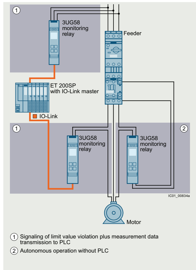
Use of monitoring relays for IO-Link
