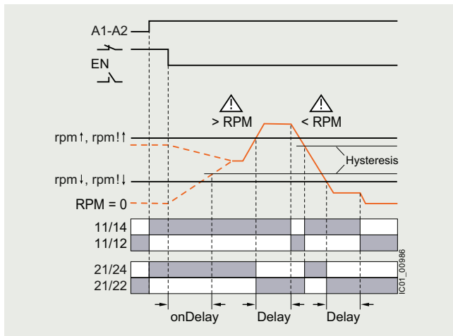
Range monitoring with enable input for 3UG5651
