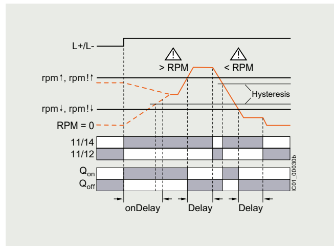
Range monitoring with enable input for 3UG5851
