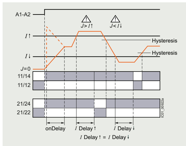
Range monitoring of current
