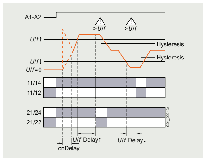
Range monitoring of voltage or frequency
