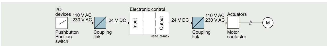
Application example motor controller
